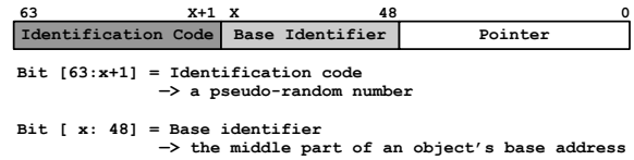
Figure 2: The object ID used in ViK.
